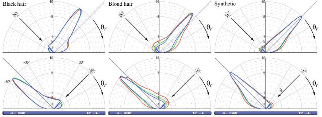
Figure 3.2: The scattering behaviour in the incidence plane (longitudinal scattering). For human hair the specular reflection is shifted towards the root by a few degrees. For synthetic hair no shifted highlight is visible, because synthetic hair doesn't consist of tilted cuticle scales.
