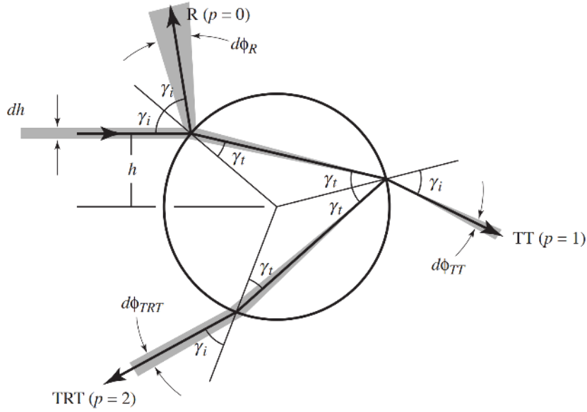
Figure 3.5: Cross section of a hair fiber showing the different scattering modes. Taken from Marschner et al. [11]
