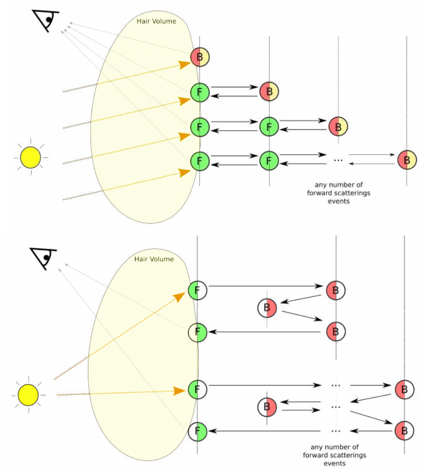
Figure 3.8: Visualization of the average backscattering attenuation A_b . The circles represent the cross section of the hair fibers. The color coded half circles represent the scattering event taking place, with red being a backward scattering event and green a forward scattering event, also indicated by B and F respectively. The orange ray correspond to the incident light from the light source. It represent the global illumination passing through the hair volume reaching the local neighborhood. The dual scattering method takes into account only one or three backscatter events. All permutations of one backscatter event ( A_1(\theta) ) is displayed in the top figure and all permutations for three backscatter events ( A_3(\theta) ) is displayed in the bottom figure. It is clear to see that the amount of forward scattering events may go to infinity, but that the amount of backscattering events is limited to one or three. This leads to the infinite series that can be written as shown in equation 3.25.
