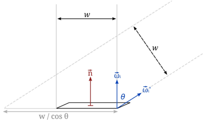
Figure 2.4: As the incoming light hits the surface at a larger angle, the irradiance decreases because the same amount of light will be spread over a greater surface area.
