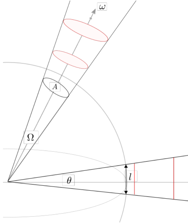
Figure 2.3: Graphical representation of angles and solid angles. \theta represents a two-dimensional angle. If the circle is considered a unit sphere, then the length of line l equals \theta radians and it subtends the red lines on the right. The solid angle \Omega is a three-dimensional angle represented by a cone. At the unit sphere, the solid angle represents a surface area A . The red disks shown on the outside represents three-dimensional objects that are subtended by the solid angle \Omega . Larger objects can be subtended by the same solid angle as they are placed farther away from the center of the sphere. As the solid angle becomes infinitely small, we obtain a direction vector \omega .
