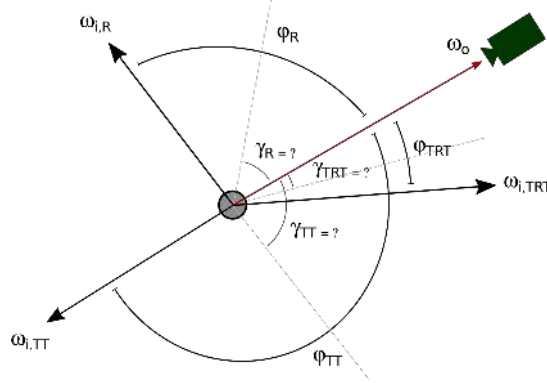
Figure 3.6: Visualization of the root finding strategy. The relative difference angle \phi_p between rays \omega_o and \omega_{i,p} is known by computing the difference of the azimuthal spherical coordinates. The Marschner model can be evaluated when the roots are known. The roots h can be found by solving the roots of equation 2p\gamma_t - 2\gamma_i + p\pi - \phi_p = 0 . Knowing \gamma_i will trivially give h .
